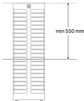
Figure 2. Installing HUUM STEEL electric heater inside the sauna bench
